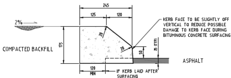
SEMI-MOUNTABLE - TYPE 1
